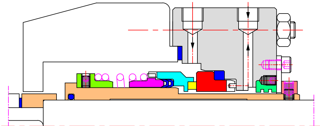
80 SERIES SINGLE SPRING MECHANICAL SEAL TYPE 8222 CARTRIDGE ARRANGEMENT WITH DIFFERENT API PLAN 11& 62
